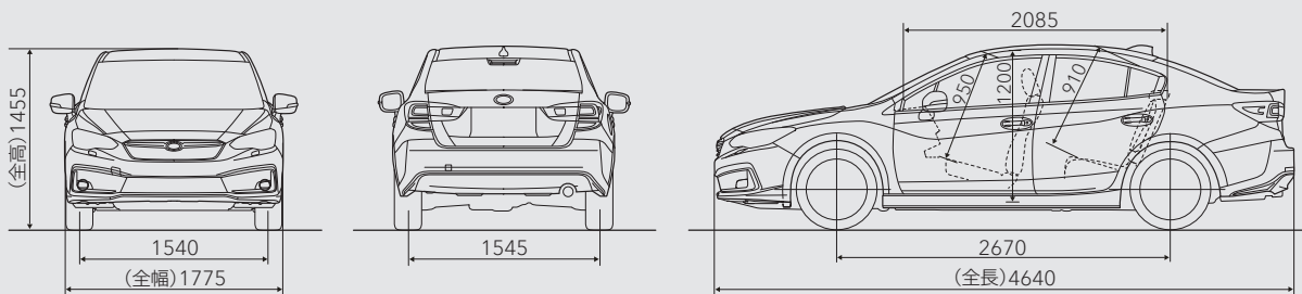
3面図(2.0i-S EyeSight) 単位: mm
