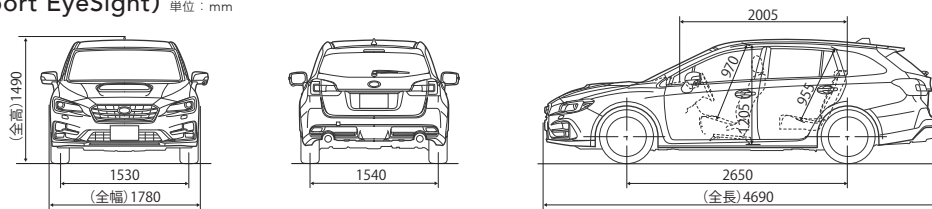
3面図(1.6STI Sport EyeSight) 単位: mm
